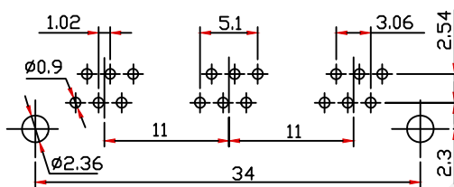
PCB Layout
